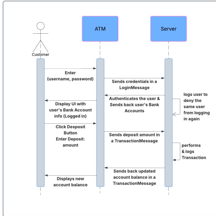
Main Sequence Diagram
